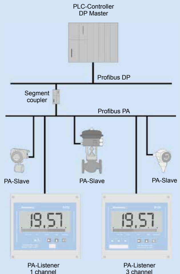
Application example of a Profibus PA - D122PA
