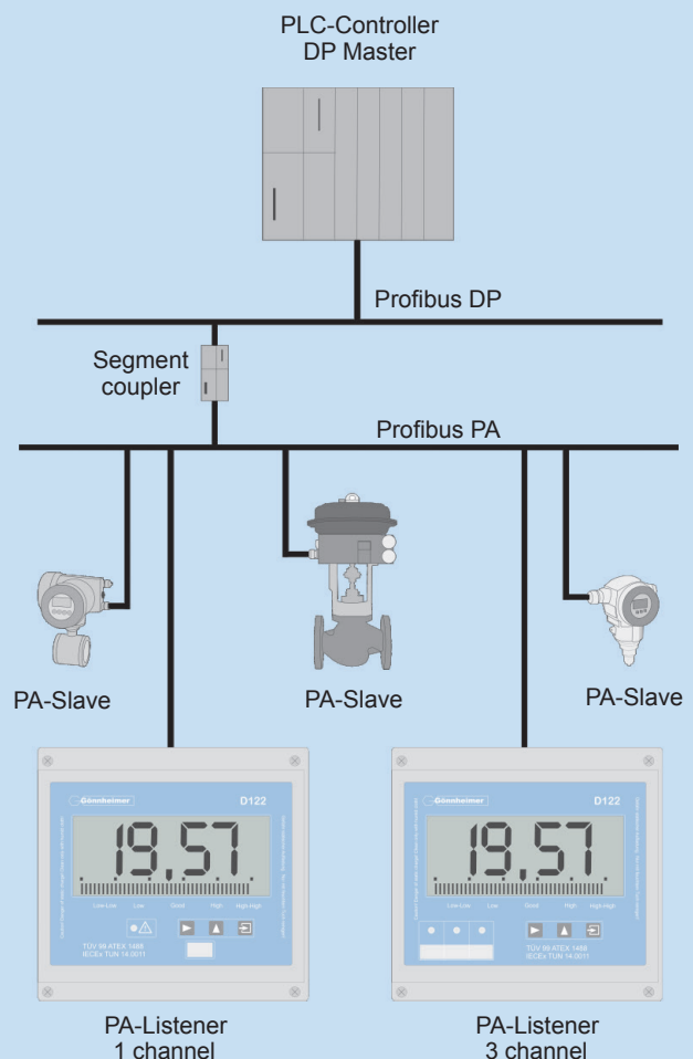
Application example of a Profibus PA - D122PA
