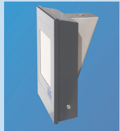
PC100 19", touch, ceiling mounting
